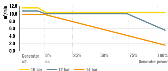
Flow rate in generator mode
